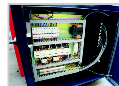
Electrical Cabinet 电器箱
