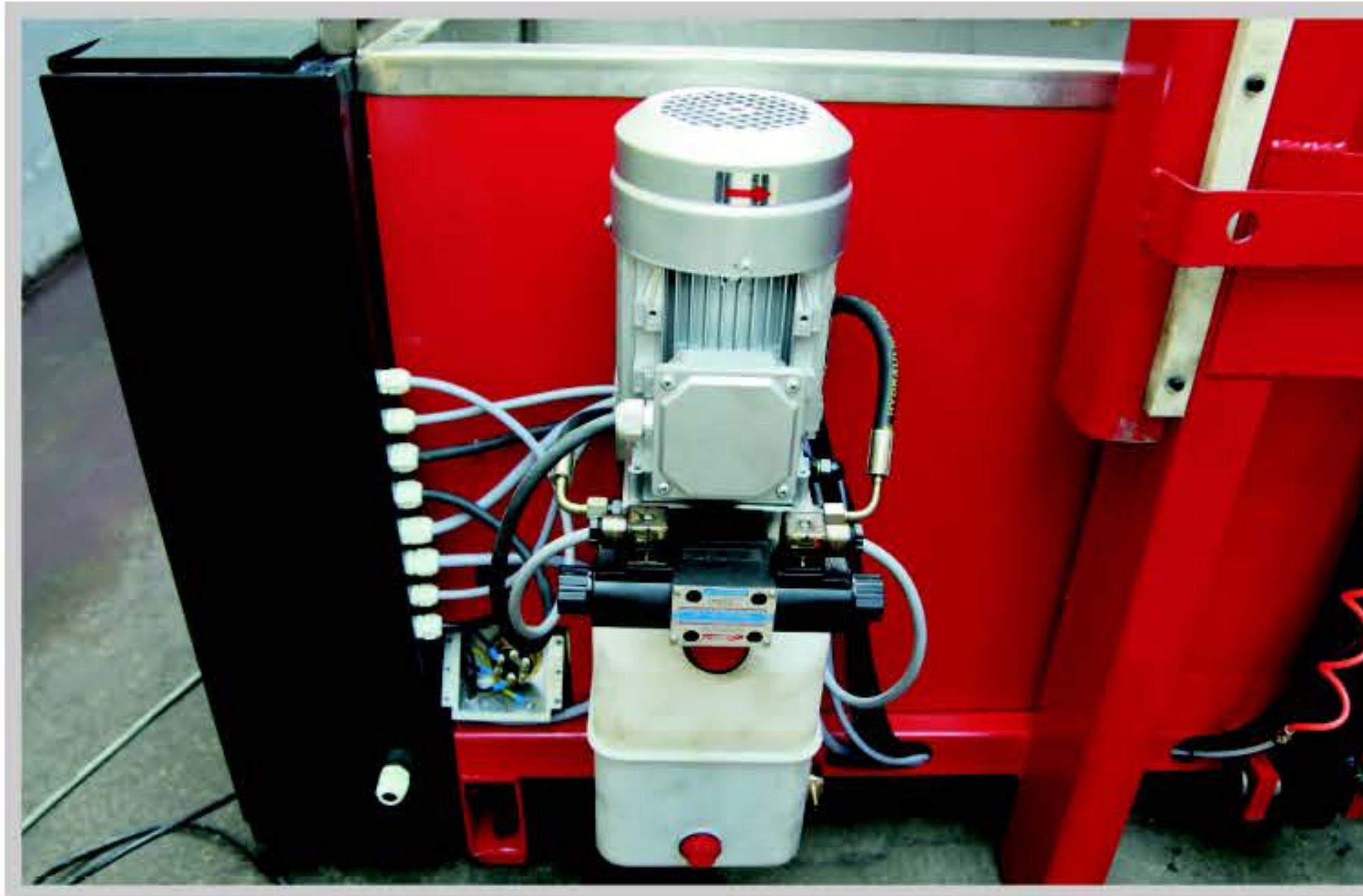
液压站/Hydraulic Unit
