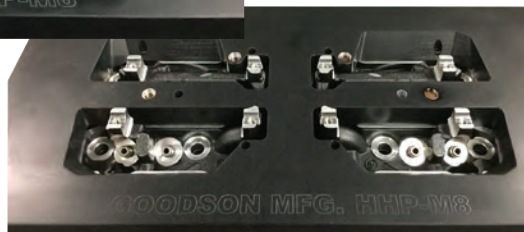
Below: View of the underside of the plate with heads mounted
